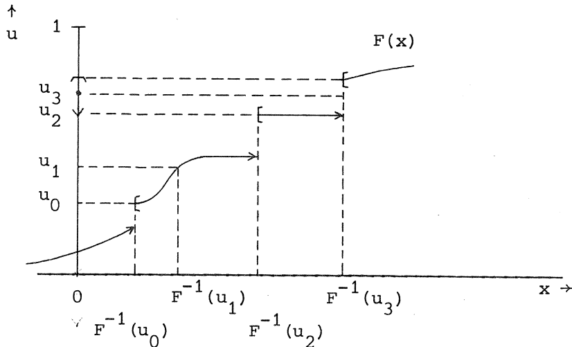
Fig.1 Illustration of F^{-1}
